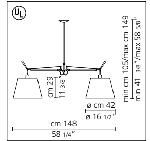
Tolomeo double shade suspension 17" diffuser
