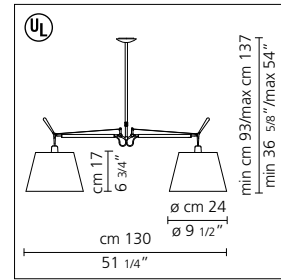
Tolomeo double shade suspension 10" diffuser
