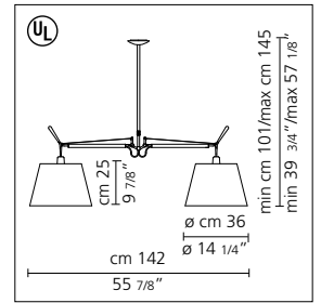
Tolomeo double shade suspension 14" diffuser
