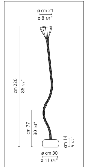
Pipe floor
