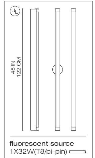
chrome end caps with a white round junction box cover plate
